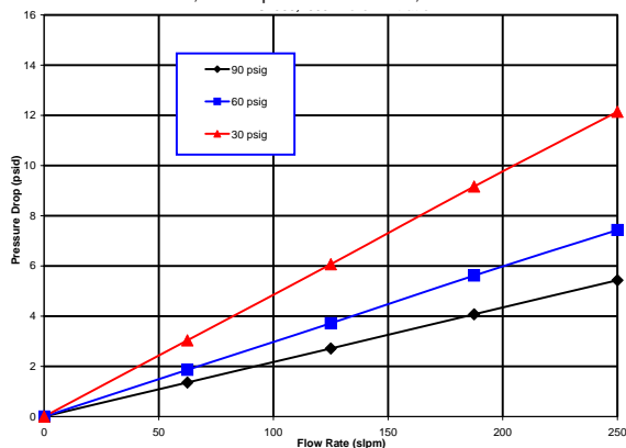
Pressure Drop vs. Flow Rate MC1500, 0.003 µm Particle Filter, tested in N 2
